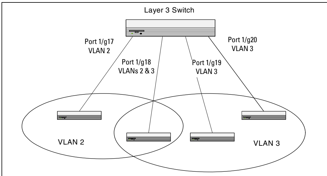
Figure 3-1. VLAN Example Network Diagram
